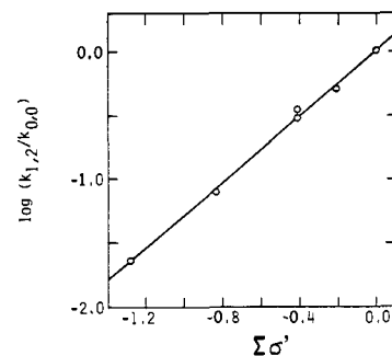
Figure 1. Plot of \log(k_{1,2}/k_{0,0}) values for m - and p -methyl derivatives of bibenzyl vs. \Sigma\sigma' values from equilibrium acidities of toluene, m -xylene, and p -xylene (eq 10).
