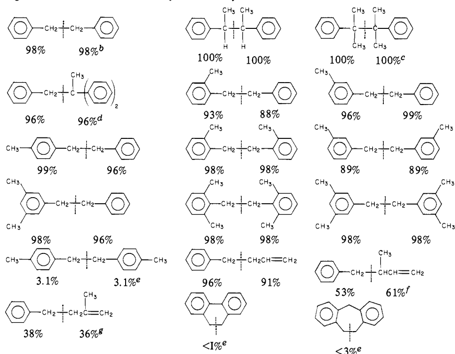
Chart I. Yields in Cleavage of Carbon-Carbon Bonds of Hydrocarbon by Cs-K-Na in THF at -75\text{ }^{\circ}\text{C}^a
